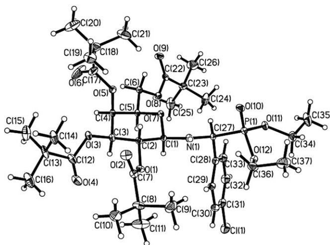
Figure 2. ORTEP presentation of the crystal structure of 4e , with 20% probability displacement ellipsoids.
