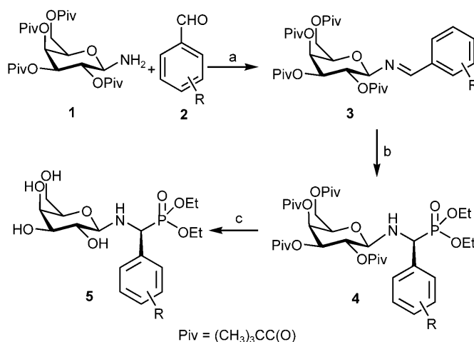
Scheme 1. Reagents and conditions: (a) i -PrOH, 2–3 drops of acetic acid, room temperature, 0.5 h; (b) 1.5 equiv. \text{HP(O)(OEt)}_2 , 2 equiv. \text{BF}_3 \cdot \text{Et}_2\text{O} , THF, room temperature, 2.5–4 h; (c) 0.5 M \text{NaOMe/MeOH} , room temperature, 2 d, 0.01 \times 7(732) , \text{H}^+ .
