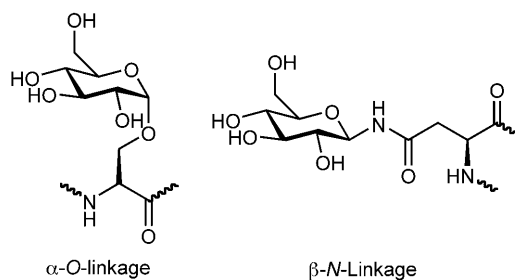
Figure 1. \alpha -O-Glycosidic and \beta -N-glycosidic linkages between carbohydrate and peptides
