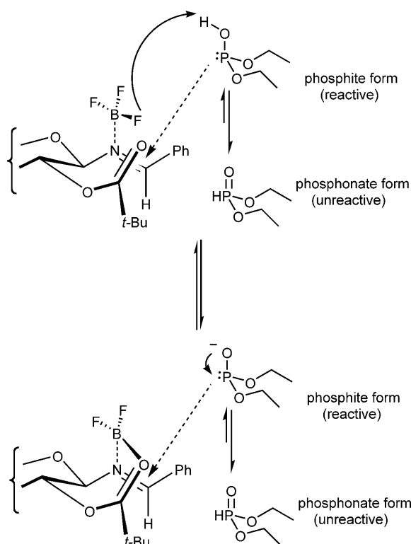
Figure 3. Plausible reaction mechanism.
